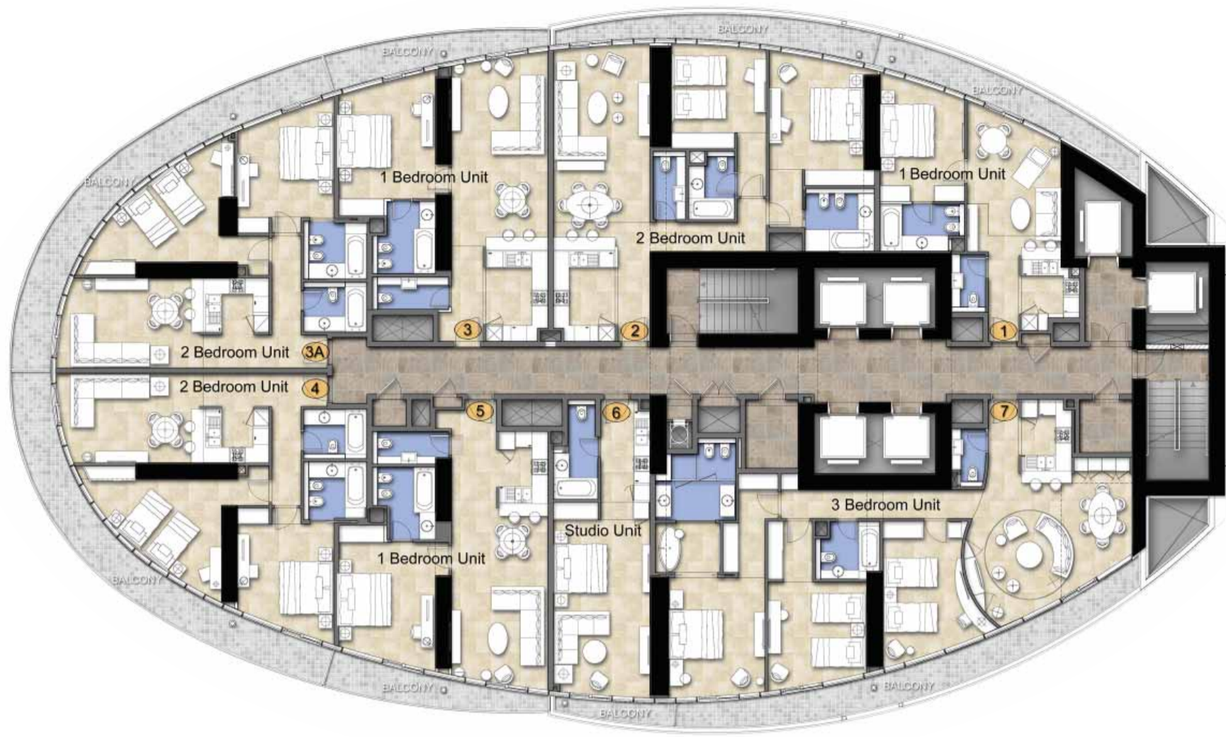
9TH TO 11TH & 26TH TYPICAL FLOOR
